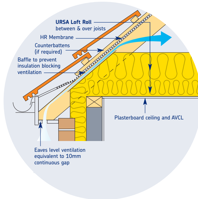
Figure 3 – Ventilated Roof Void
