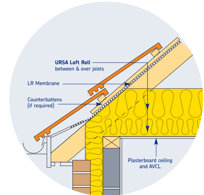
Figure 4 – Non-Ventilated Void
