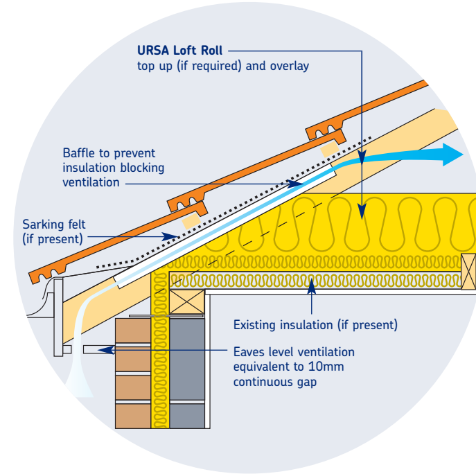
Figure 5 – Loft Insulation Upgrade
